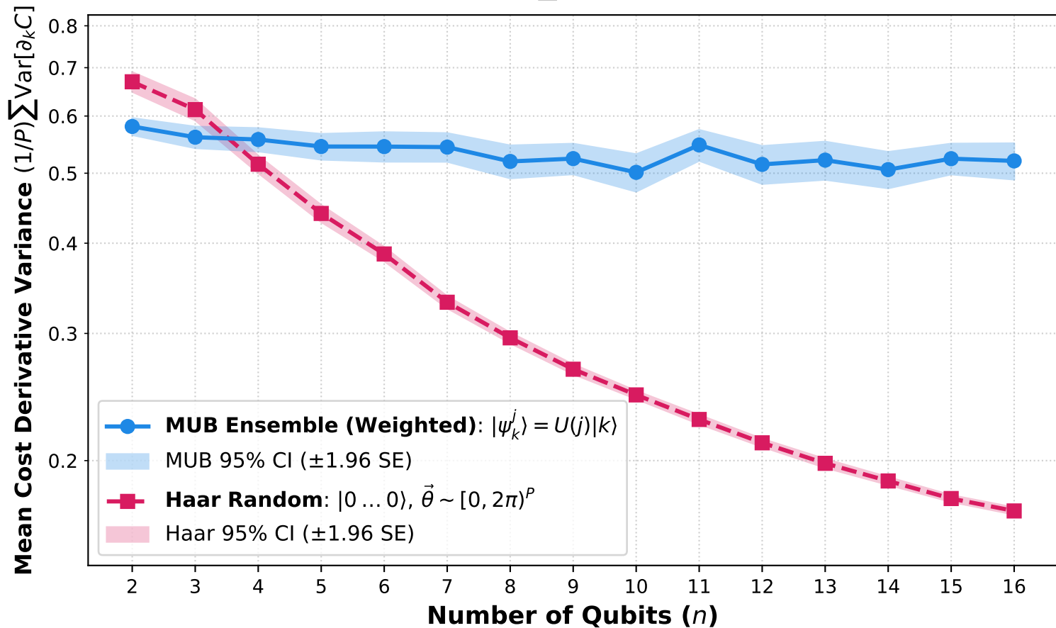
VQE Mean Cost Derivative Variance vs. System Size n 1D TFIM Model ( J = 1.0, h = 1.0 ) HEA Depth L = 2n , (1/P)\sum \text{Var}[\partial_k C] ( N = 1000 samples)
