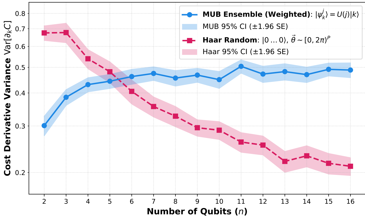
VQE Cost Derivative Variance vs. System Size n 1D TFIM Model ( J = 1.0, h = 1.0 ) HEA Depth L = 2n , Parameter \partial_{\theta_1} C
