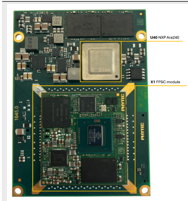
图 3: phyVIP (Kinara) Components (top)
