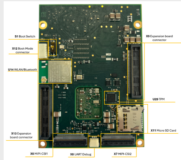
图 4: phyVIP (Kinara) Components (bottom)
