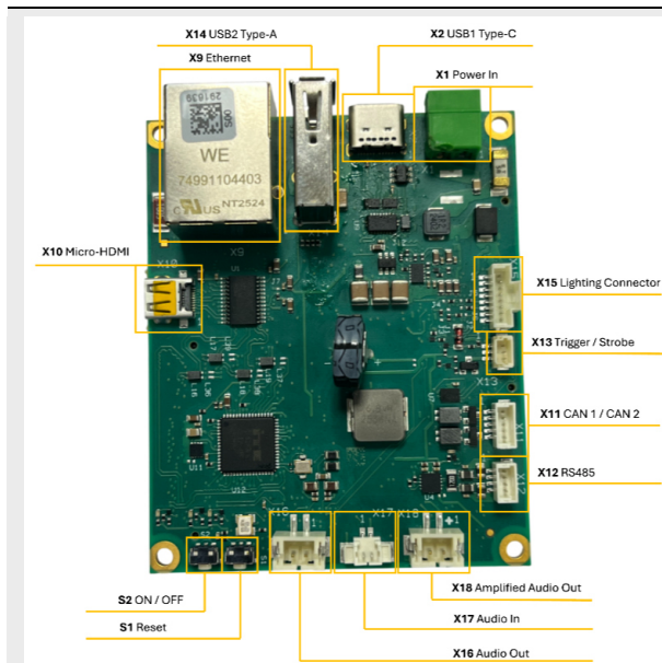
图 5: phyVIP PEB-B-006 expansion board Components (top)
