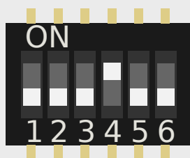
Fig. 8: UART1 RS485
