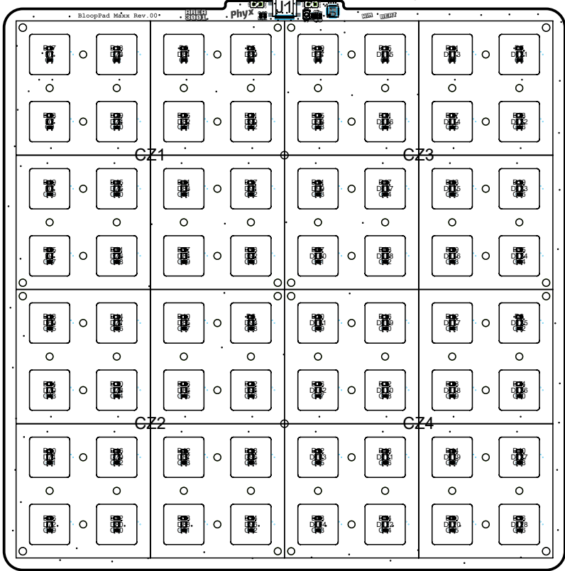
View from Top side (Scale 1:2)
