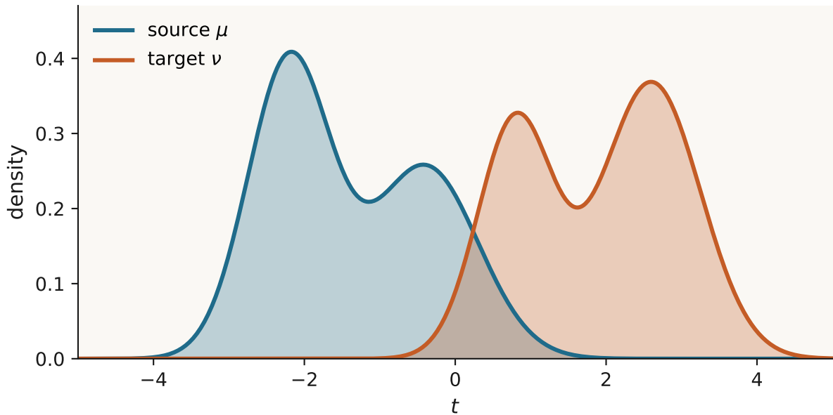
Two equal-mass densities on the line
