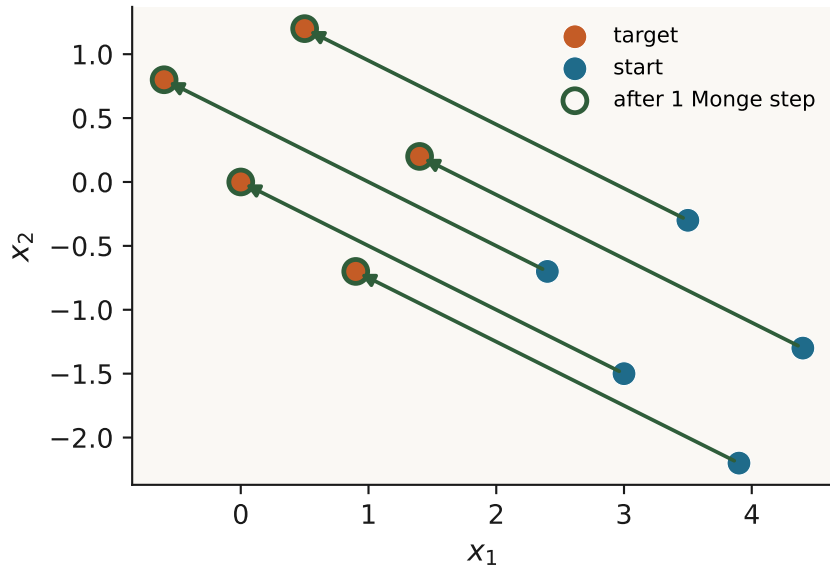
Monge: one step \approx exact translation
