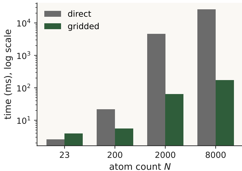
Value + gradient, L = 24
