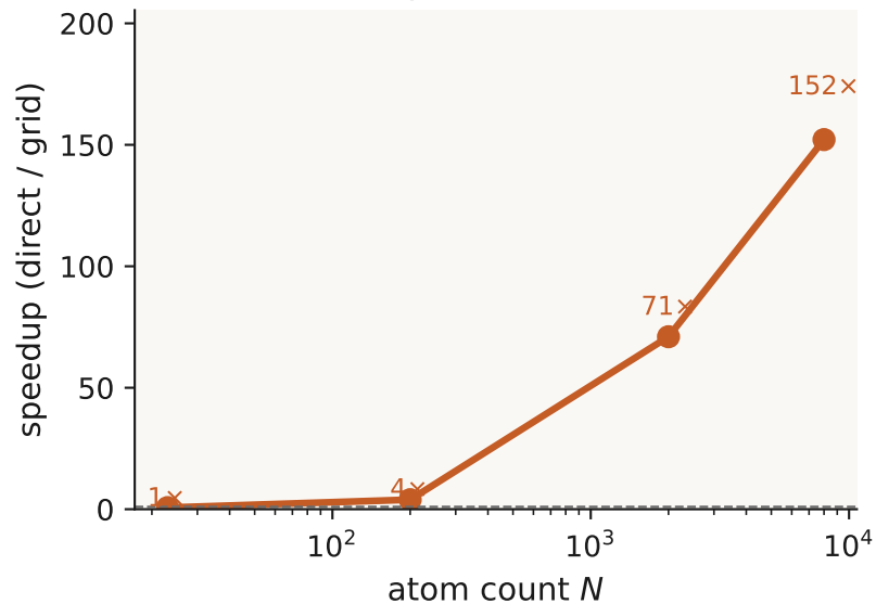
Gridded wins past a few dozen atoms
