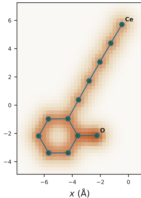
ADMM OT+L1+ P_{\text{restr}} RMSD 0.027 Å
