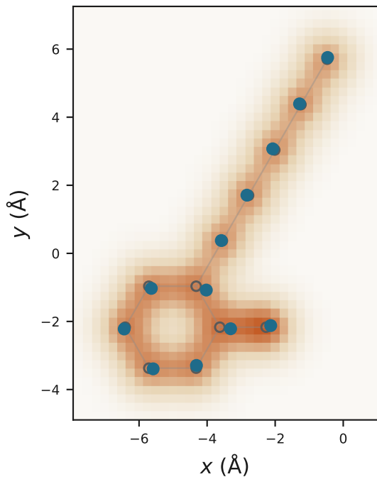
unlabelled free cloud (shuffled indices after OT)
