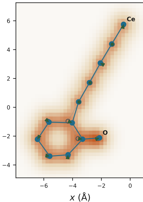
after Namer.assign label-RMSD 0.15 Å · restr 0.12
