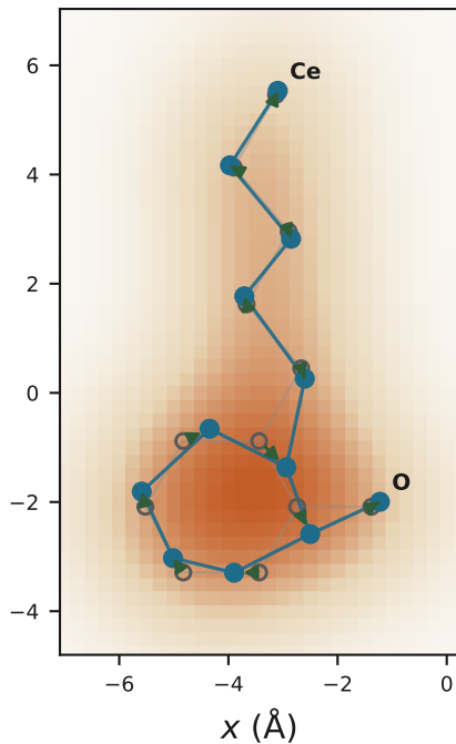
after Namer.assign label-RMSD 0.36 Å · restr 0.23
