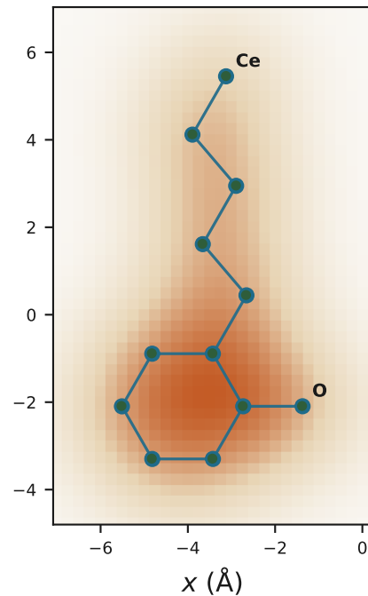
ADMM OT+L1+ P_{\text{restr}} RMSD 0.012 Å
