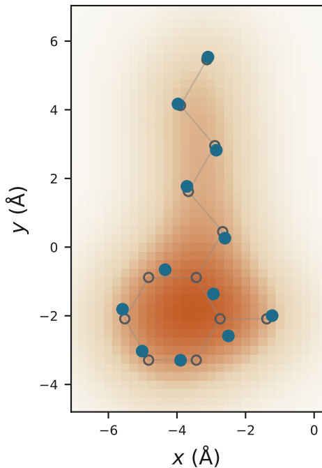
unlabelled free cloud (shuffled indices after OT)
