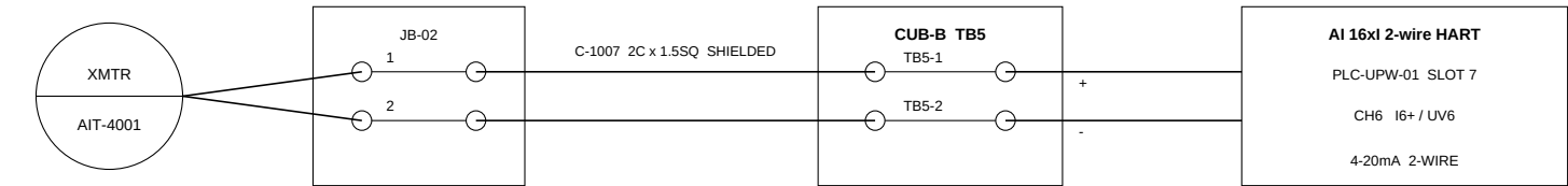
UPW TANK RESISTIVITY
