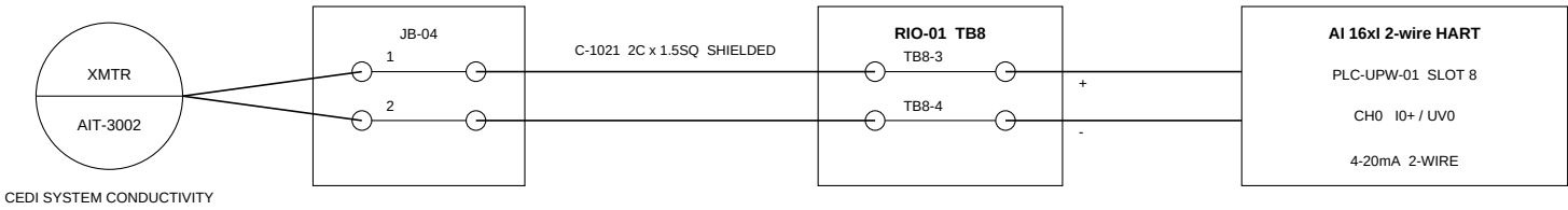
CEDI SYSTEM CONDUCTIVITY
