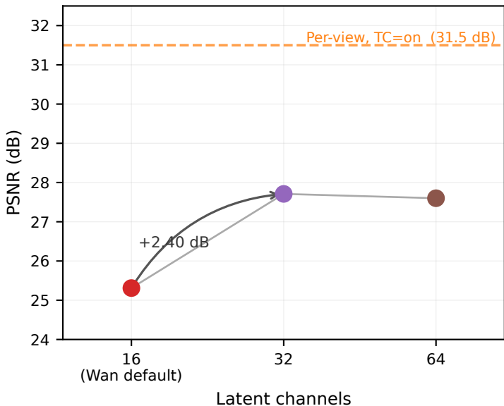
Latent Width Ablation (fused, TC=on)
