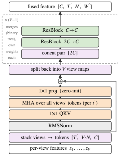
(a) Multi-view attention + tree merge (default)
