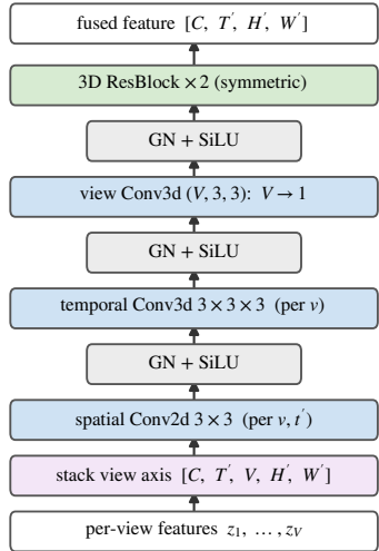
(c) Factorized 4D convolution
