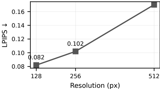
Perceptual error vs resolution 0.170
