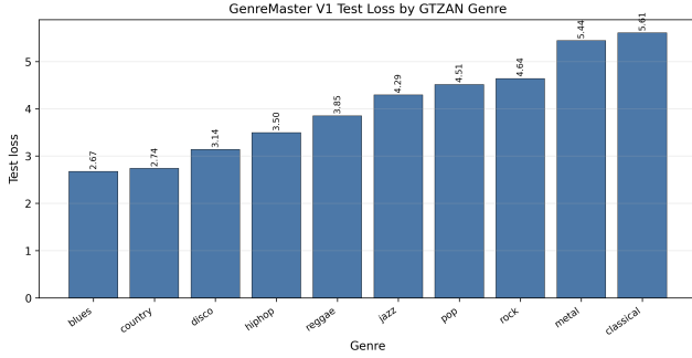
Fig. 3. Per-genre test loss for V1 on GTZAN.
