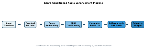
Fig. 1. Genre-conditioned neural audio enhancement pipeline. Input audio is encoded into spectral features, combined with learned genre embeddings via FiLM conditioning, and used to predict DSP parameters for differentiable audio transformations.
