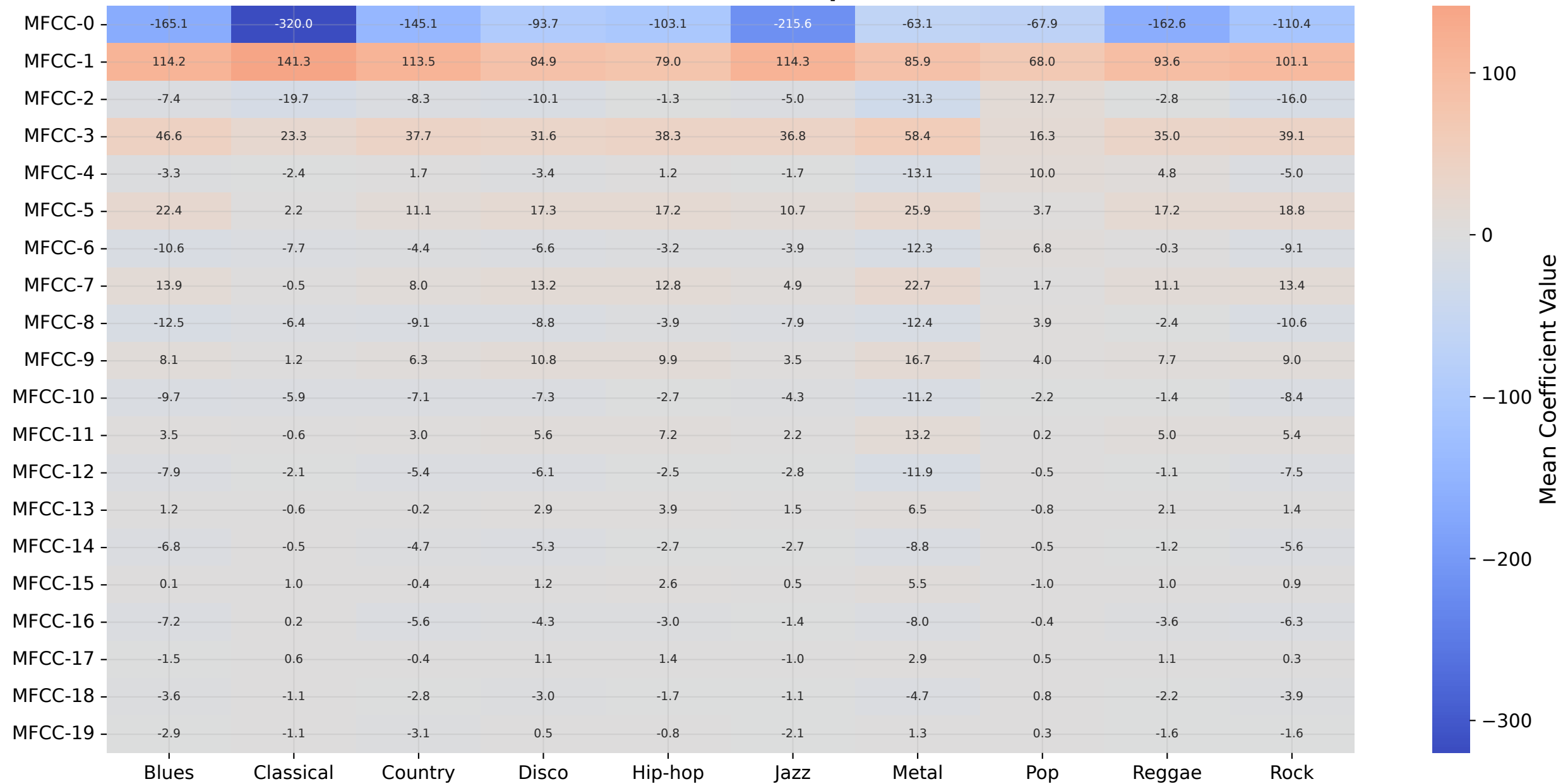
Mean MFCC Coefficients per Genre
