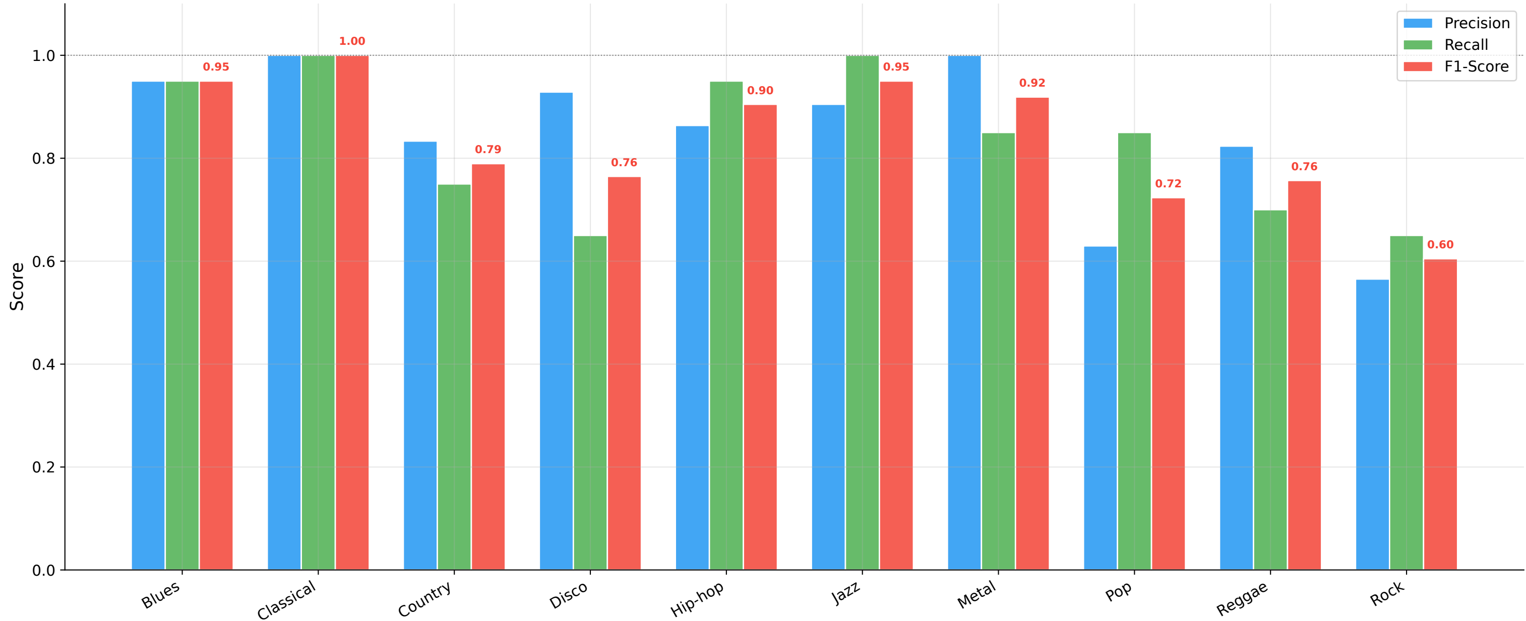
Per-Class Classification Metrics
