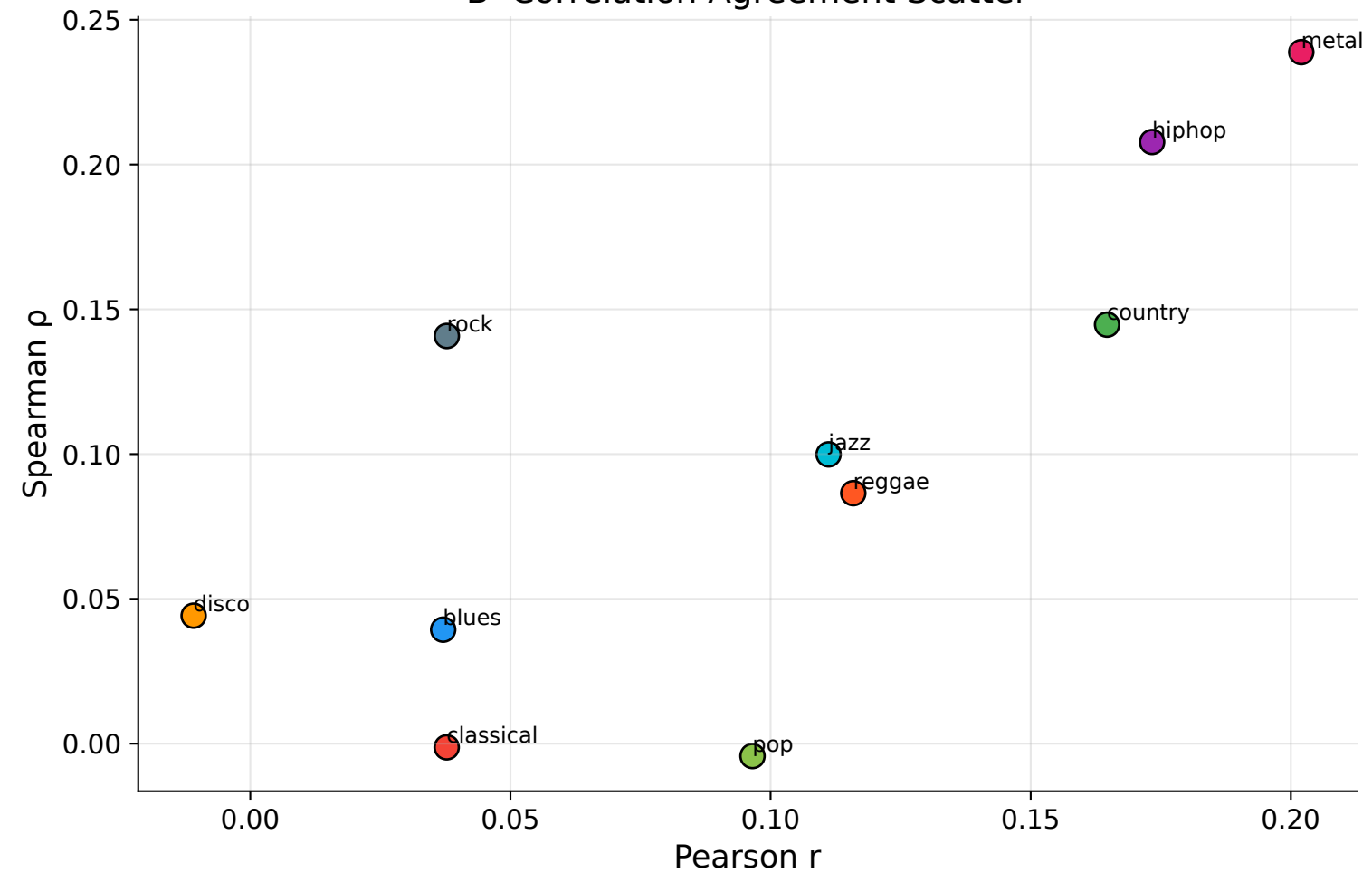
B Correlation Agreement Scatter
