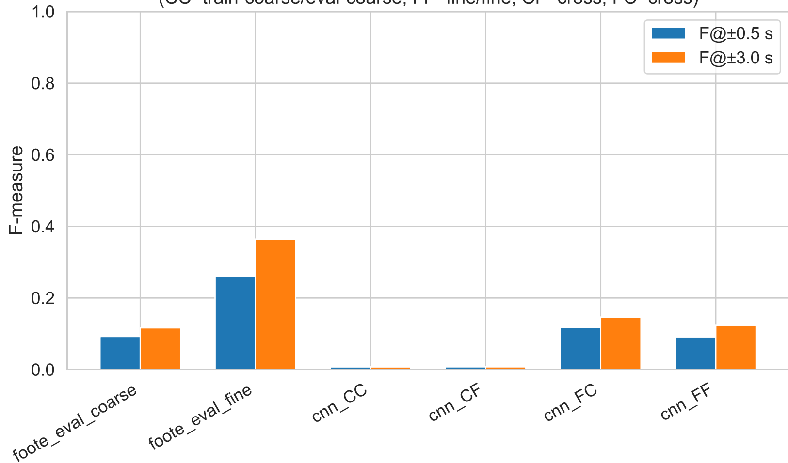
Boundary Detection: Level-Conditional Results (CC=train-coarse/eval-coarse, FF=fine/fine, CF=cross, FC=cross)
