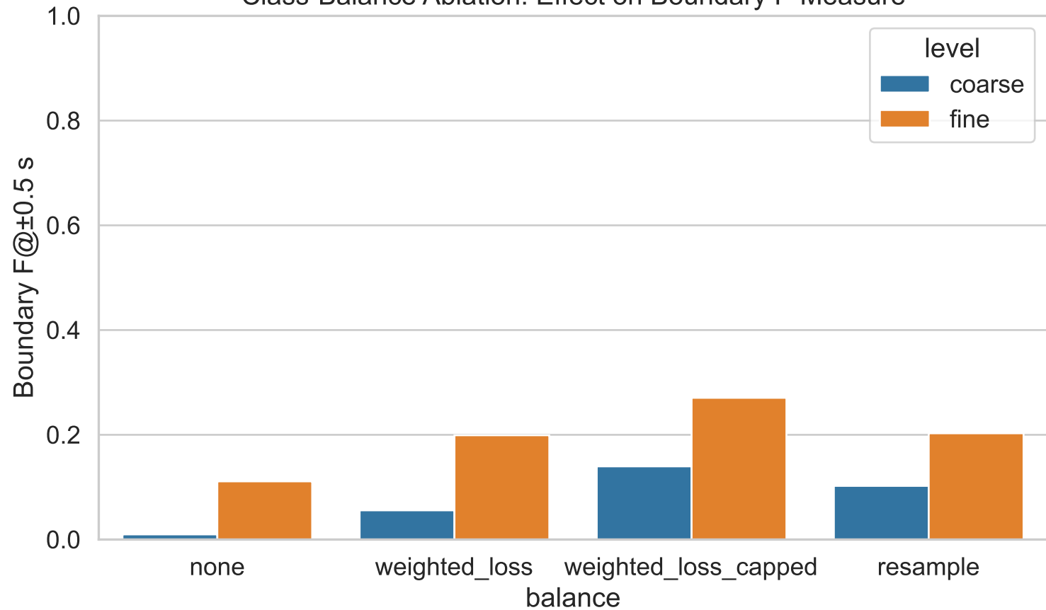
Class-Balance Ablation: Effect on Boundary F-Measure
