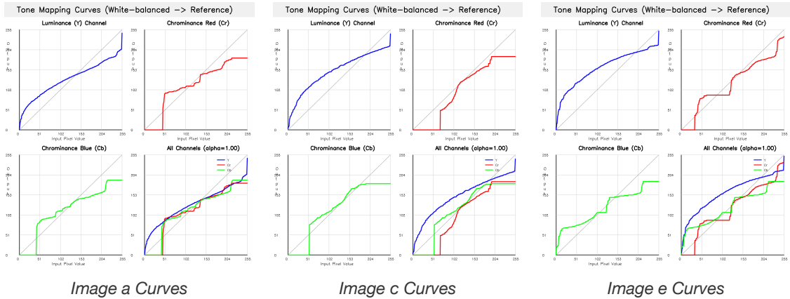
Figure 10: Tone curve comparison - Image a shows moderate correction, Image c minimal adjustment, Image e aggressive transformation
