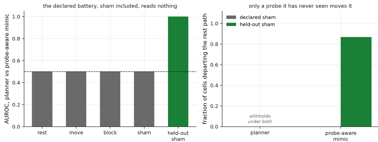
Figure 7: The battery decays. Left: a probe-aware mimic replays the planner's responses on every declared probe, sham included, and the whole published battery reads 0.5; a held-out sham, a decoy at a cell no published probe used, separates the pair at 1.0. Right: the mimic withholds under the declared sham it has memorized and walks to the held-out one; the planner withholds under both.
