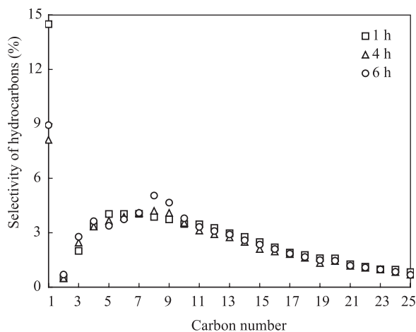
Fig. 4. Effect of time-on-stream on the selectivity of the products. Reaction conditions: T=240\text{ }^{\circ}\text{C} , P_{\text{total}}=4.5\text{ MPa} , P_{(\text{CO}+\text{H}_2)}=1.0\text{ MPa} , P_{\text{hexane}}=3.5\text{ MPa} and W/F=5\text{ g cat. h/mol} .
