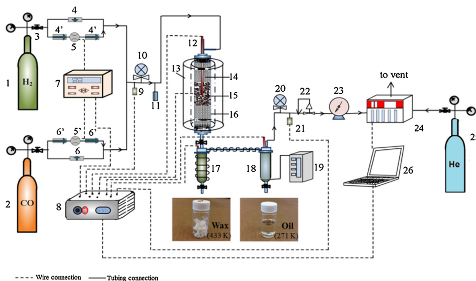
Fig. 1. The schematic diagram of fixed-bed reactor (FBR) system. (1) Hydrogen cylinder; (2) carbon monoxide cylinder; (3)(3') pressure regulators; (4)(4') valves; (4')(6') by-pass valve; (5) mass flow controller; (7) CM-400/scanner; (8) automatic controller/scanner system; (9) front pressure sensor; (10) front pressure gauge; (11) safety valve; (12) thermocouple; (13) furnace; (14) sand; (15) catalyst; (16) fixed-bed reactor; (17) hot trap; (18) cold trap; (19) chiller; (20) back pressure sensor; (21) back pressure gauge; (22) back pressure regulator; (23) wet gas flow meter; (24) gas chromatography; (25) carrier gas He; (26) computer.
