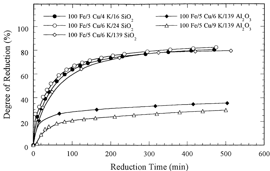
Fig. 2. Isothermal reduction behavior in hydrogen at 280 °C.
