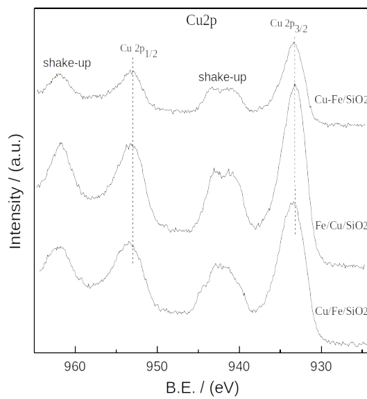
Fig. S2. XPS spectra for Cu 2p of the calcined catalysts.
