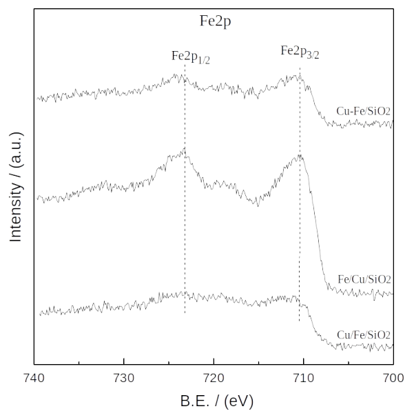
Fig. S3. XPS spectra for Fe 2p of the calcined catalysts.
