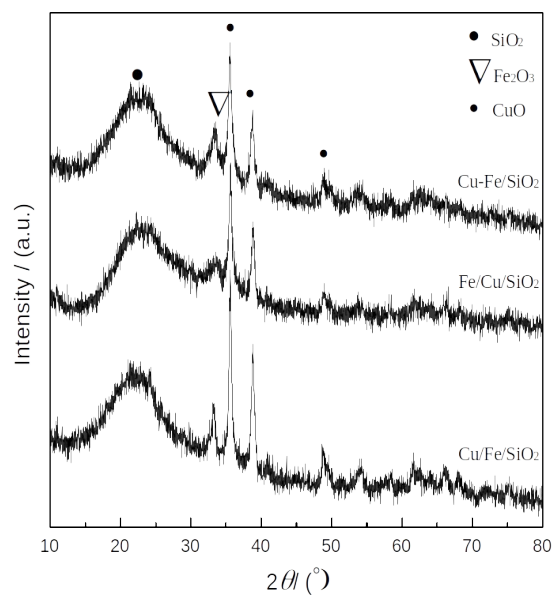
Fig. S1. XRD patterns of the calcined catalysts.
