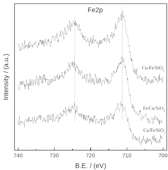
Fig. S4. XPS spectra for Fe 2p of the reduced catalysts.
