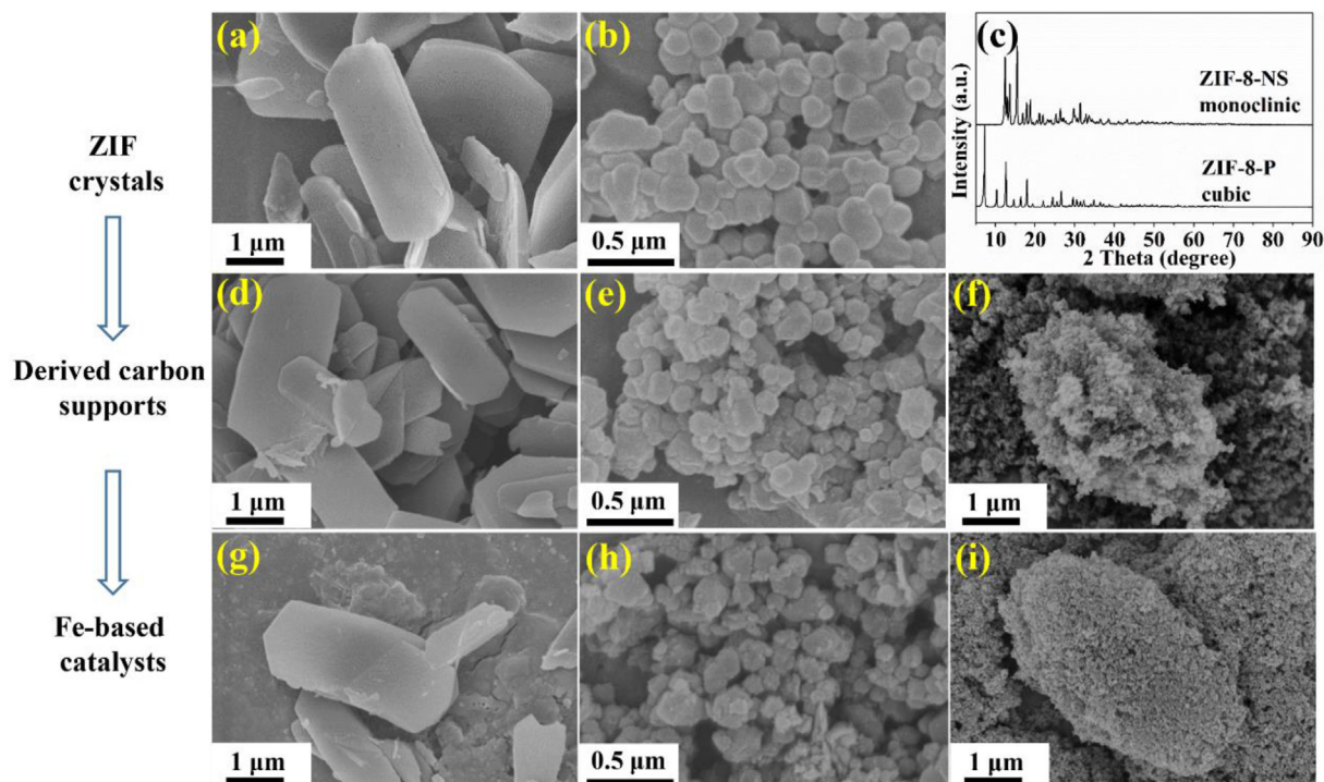
Fig. 2. SEM images (a–b) and XRD patterns (c) of ZIF crystals: ZIF-8-NS and ZIF-8-P; SEM images of derived carbon supports (d–f) and corresponding Fe-based catalysts (g–i): CNS(1000), CP, AC and Fe/CNS(1000), Fe/CP, Fe/AC. (A colour version of this figure can be viewed online.)
