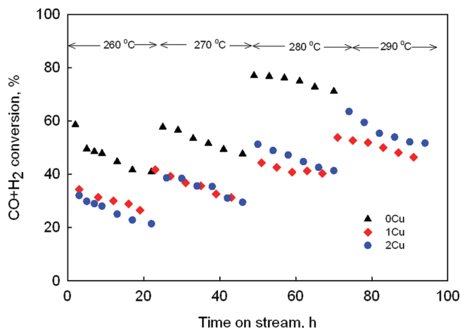
Figure 2. Change of syngas conversion with time on stream over Fe-K/AC catalysts with and without Cu. Other reaction conditions: 300 psig, 3 nL (g of catalyst) -1 h -1 , and \text{H}_2/\text{CO} = 0.9 .
