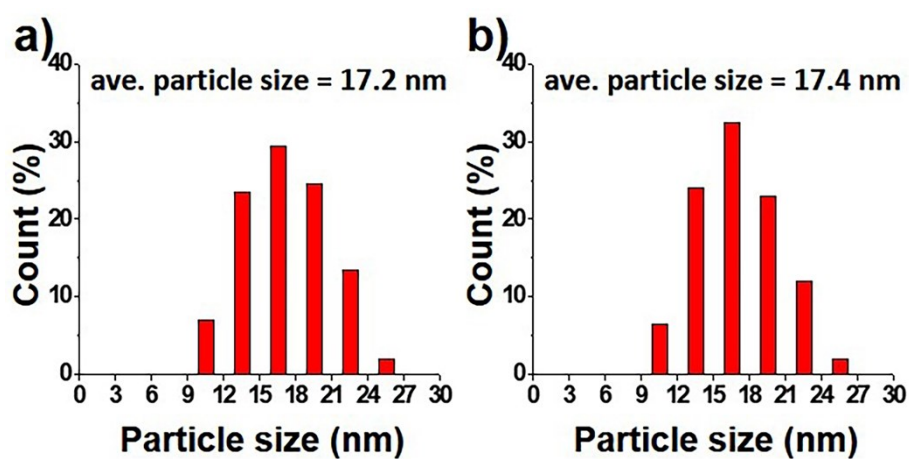
Figure S2. Particle size distributions of (a) K-free \text{Fe}_5\text{C}_2 nanoparticles and (b) K-doped \text{Fe}_5\text{C}_2 nanoparticles in each catalyst. More than 200 particles were counted for the sample.
