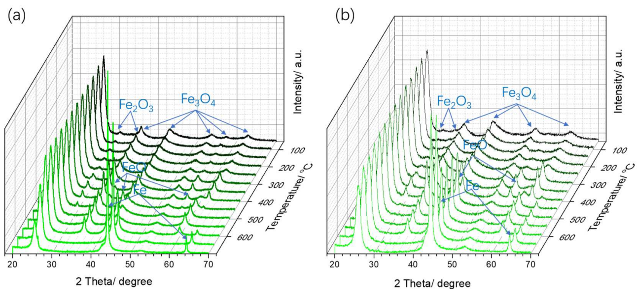
Fig. S15: In-situ XRD profiles of the iron-based catalysts (5% H 2 /N 2 ): (a) Fe/CNT, (b) FeBi/CNT.
