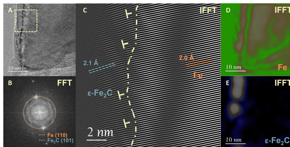
Fig. 4. Observation of \epsilon (')-carbide formation by environmental TEM. A well-ground sample was in situ reduced in a \text{H}_2 flow at 430^\circ\text{C} for 20 hours. Subsequently, the sample was exposed to a synthesis gas flow ( \text{H}_2/\text{CO} = 2.4/1.2 ) at 170^\circ\text{C} for 20 min. During this dwell, HRTEM images were taken. (A) HRTEM image. (B) FFT of selected area. (C) IFFT image. (D) IFFT image of \alpha -Fe. (E) IFFT image of \epsilon - \text{Fe}_2\text{C} .
