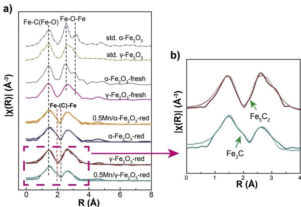
Fig. 6. The nonphase corrected, k^2 weighted Fourier-transformed in situ EXAFS spectra at the Fe K-edge of the \alpha -Fe 2 O 3 and \gamma -Fe 2 O 3 based catalysts after carburized. Dash lines denote reference samples of \alpha -Fe 2 O 3 and \gamma -Fe 2 O 3 , solid lines denote experiment spectra of iron based catalysts, and dotted lines denote fitting curves. The carburized samples were in situ treated in syngas ( H_2/CO = 1 , 15 ml/min) at 340 °C for 2 h at 1 bar.
