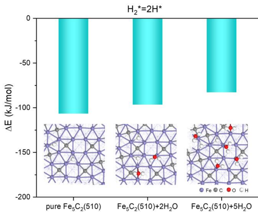
Figure S21. Dissociation energy of H_2 on pure Fe_5C_2(510) surface and H_2O -adsorbed Fe_5C_2(510) surface.
