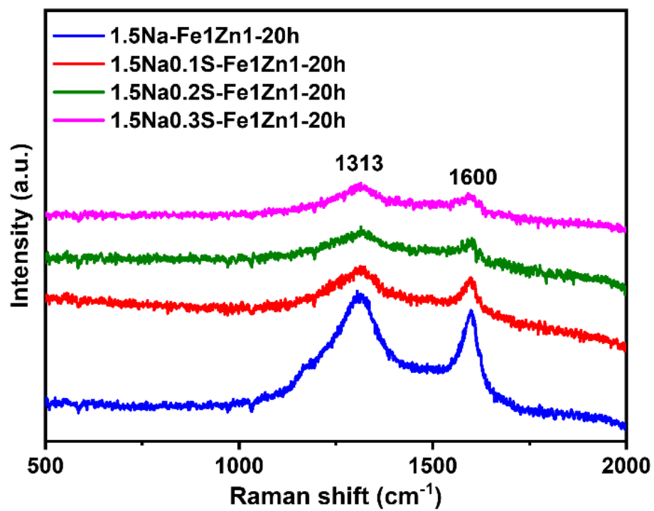
Figure S13. Raman spectra of the spent NaS-Fe1Zn1 catalysts with different Na 2 S content after CO-FTS reaction.
