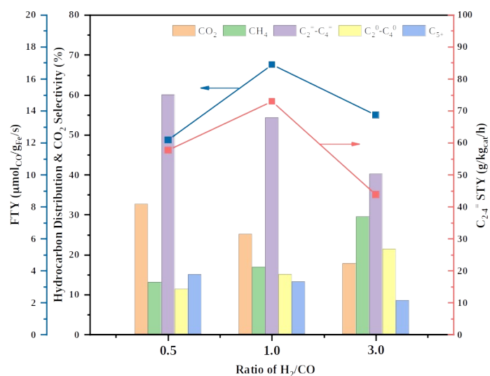
Fig. S2. Iron-time-yield (FTY), product distribution and C 2 -C 4 olefin space-time-yield (STY) at different H 2 /CO ratios (0.5, 1, 3) in syngas over a Fe-13Mn catalyst. Reaction conditions: 25mg catalyst diluted with SiC (1:3), 533K, 2.0 MPa, GHSV=4000 h -1 , TOS= 20h, syngas composition (% , v/v, H 2 /CO/N 2 ) = 30/60/10, 45/45/10, 60/20/20.
