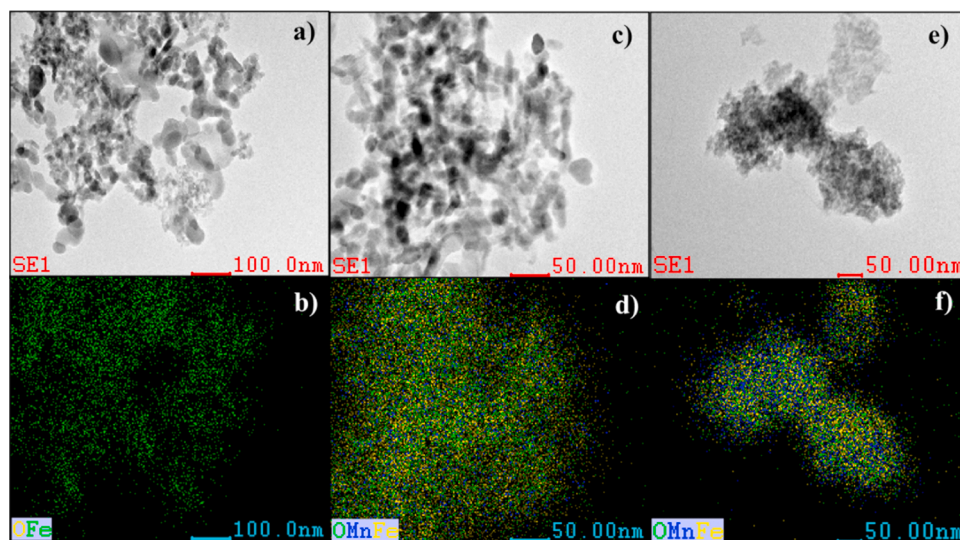
Fig. 2. TEM images and EDS mappings of the as-prepared Fe-Mn bimetallic catalysts (a-b) Fe; (c-d) FeMn(4:1); (e-f) FeMn(1:1).
