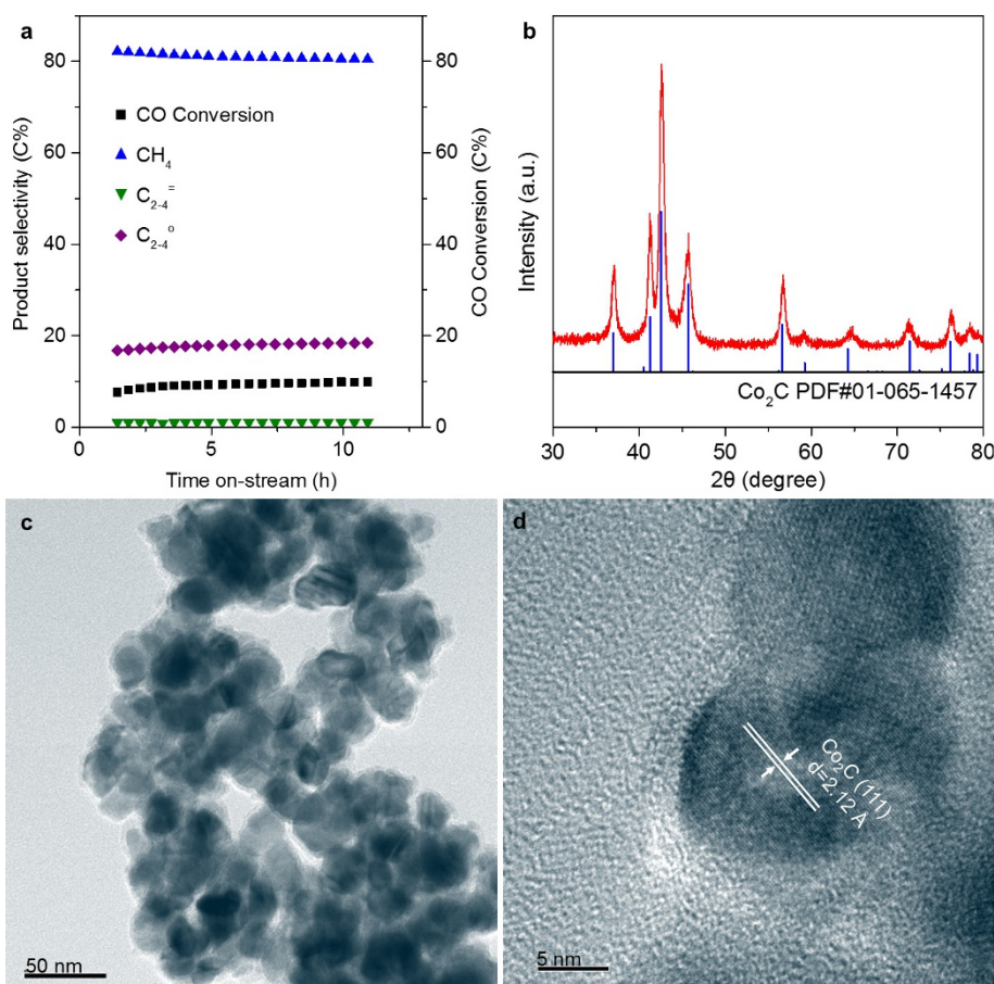
Extended Data Figure 4 | Catalytic performance and structure of \text{Co}_2\text{C} sphere-like nanoparticles. a , Catalytic performance of \text{Co}_2\text{C} sphere-like nanoparticles with time on-stream. b , XRD pattern, c , TEM image and d , high-resolution TEM image of \text{Co}_2\text{C} sphere-like nanoparticles. The \text{Co}_2\text{C} was prepared by carbonizing \text{Co}_3\text{O}_4 with pure CO at a temperature of 250 °C and at atmospheric pressure for 24 h. The reaction was performed at 250 °C, 1 bar, 2,000 \text{ml h}^{-1} \text{ g}_{\text{cat}}^{-1} , \text{H}_2/\text{CO} = 2 . The calculated
