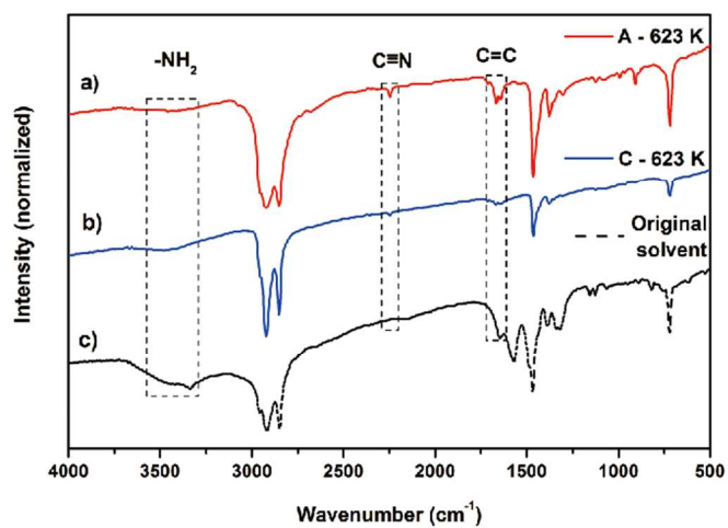
Figure S5. FTIR spectra of a) A-623 K, b) C-623 K and c) the original solvent. The frames indicate the peaks for the corresponding chemical bonds.
