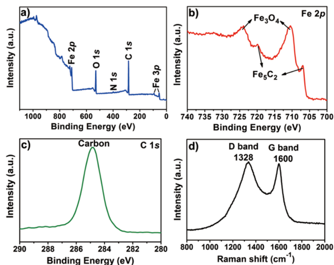
Figure 3. XPS and Raman spectra of the Fe 5 C 2 NPs. (a) XPS survey spectrum of Fe 5 C 2 NPs showing the presence of carbon and oxygen on the Fe 5 C 2 surface. (b) Fe 2p XPS spectrum, which indicates the existence of an Fe 3 O 4 phase on the Fe 5 C 2 surface. (c) C 1s XPS spectrum and (d) Raman spectrum, which suggest the coexistence of amorphous and graphitic carbon on the surface of Fe 5 C 2 NPs.
