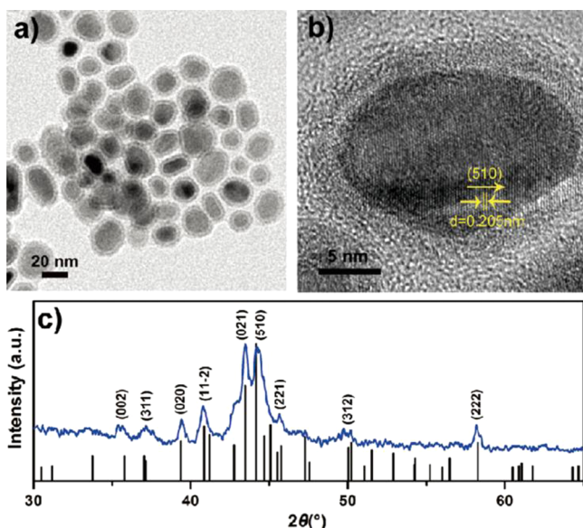
Figure 1. (a) TEM image of 20 nm Fe 5 C 2 NPs. (b) HRTEM image of a single 20 nm Fe 5 C 2 NP, which reveals that the NP has a core-shell-like structure with a well-crystallized Fe 5 C 2 core and an amorphous shell. (c) XRD pattern of 20 nm Fe 5 C 2 NPs (JCPDS no. 36-1248).
