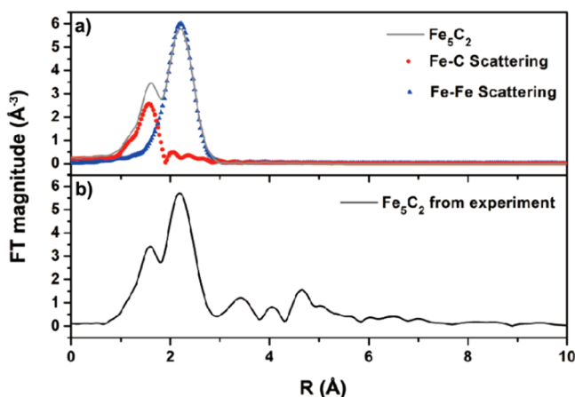
Figure 2. (a) Simulated FT-EXAFS data for Fe 5 C 2 (gray solid line) as a sum of contributions from carbon scattering (red ●) and iron scattering (blue ▲). (b) Experimental FT-EXAFS pattern obtained for the Fe 5 C 2 NPs.
