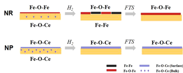
Scheme 1. Schematic Description of Structural Evolutions on Iron–Ceria Catalysts
