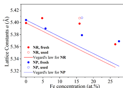
Figure 2. Lattice constants ( a ) of CeO 2 as a function of Fe concentrations for iron-ceria samples.
