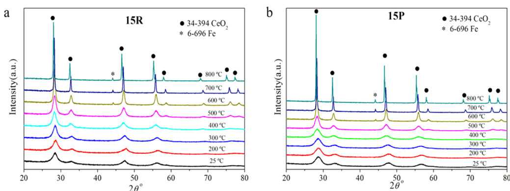
Figure 10. In situ XRD patterns of 15R (a) and 15P (b) samples under similar conditions of \text{H}_2 -TPR.
