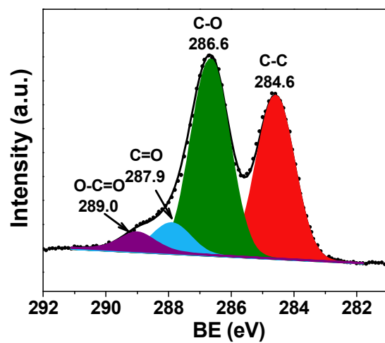
Figure S2 The C 1s XPS spectrum of GO.
