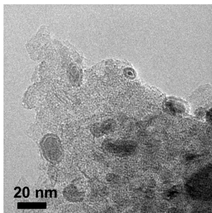
Figure S3 TEM image of the FeK1/rGO catalyst after 120 h on stream in FTO.
