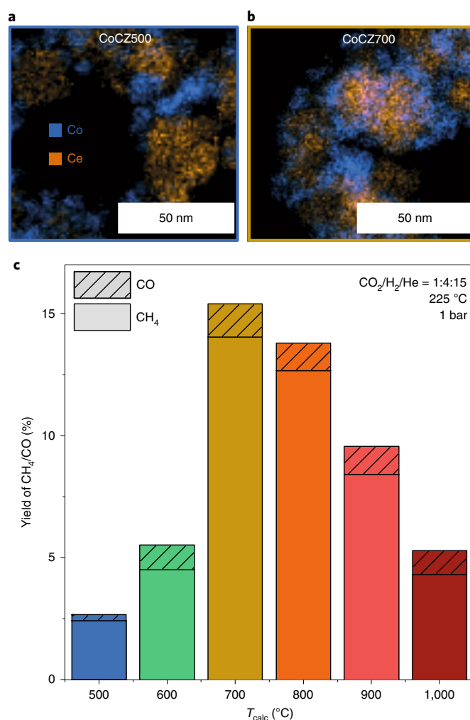
Fig. 1 | The effect of support calcination pretreatment on catalytic activity. a,b, EDX mapping of as-prepared CoCZ500 (a) and CoCZ700 (b). c, Catalytic performance at 225 °C of cobalt-based catalysts supported on CZ calcined at different temperatures ( T_{\text{calc}} ).
