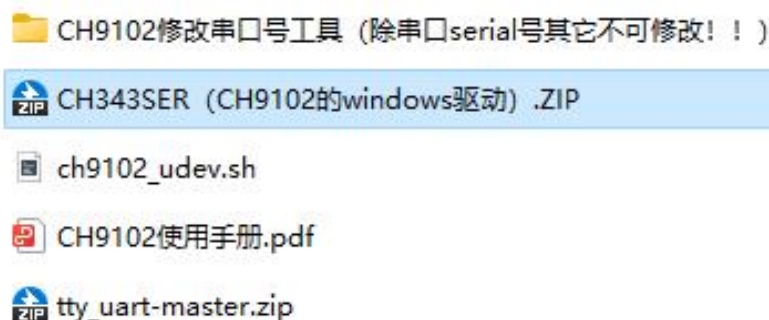
图 2-3 CH343SER
