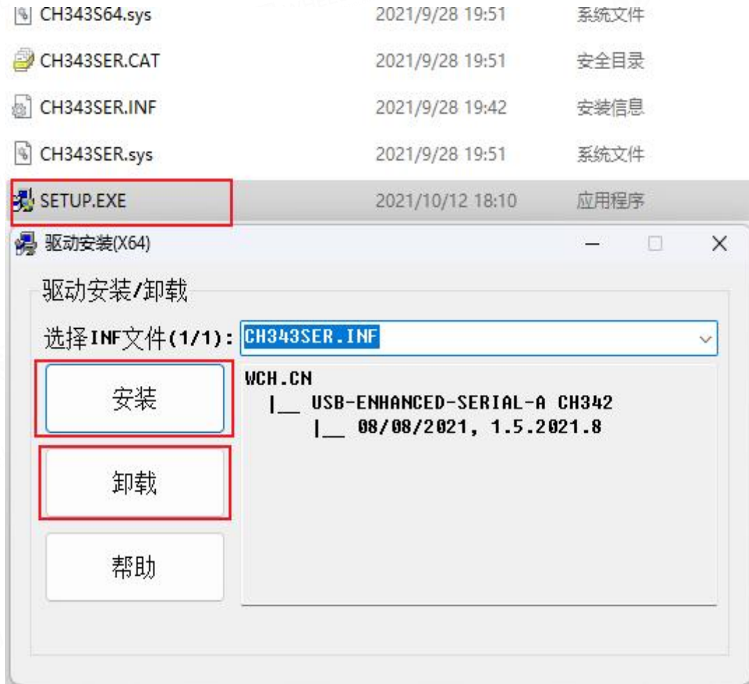
图 2-4 SETUP.EXE
