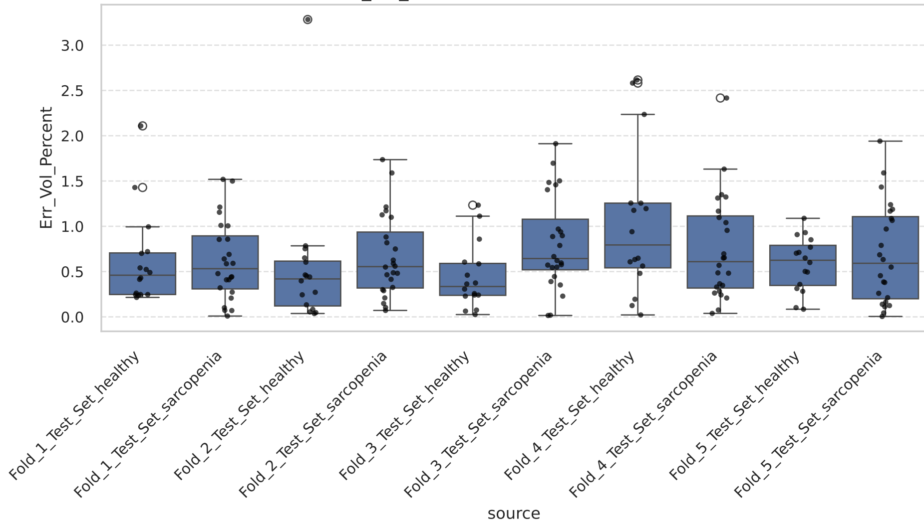
Err_Vol_Percent across folds / test sets
