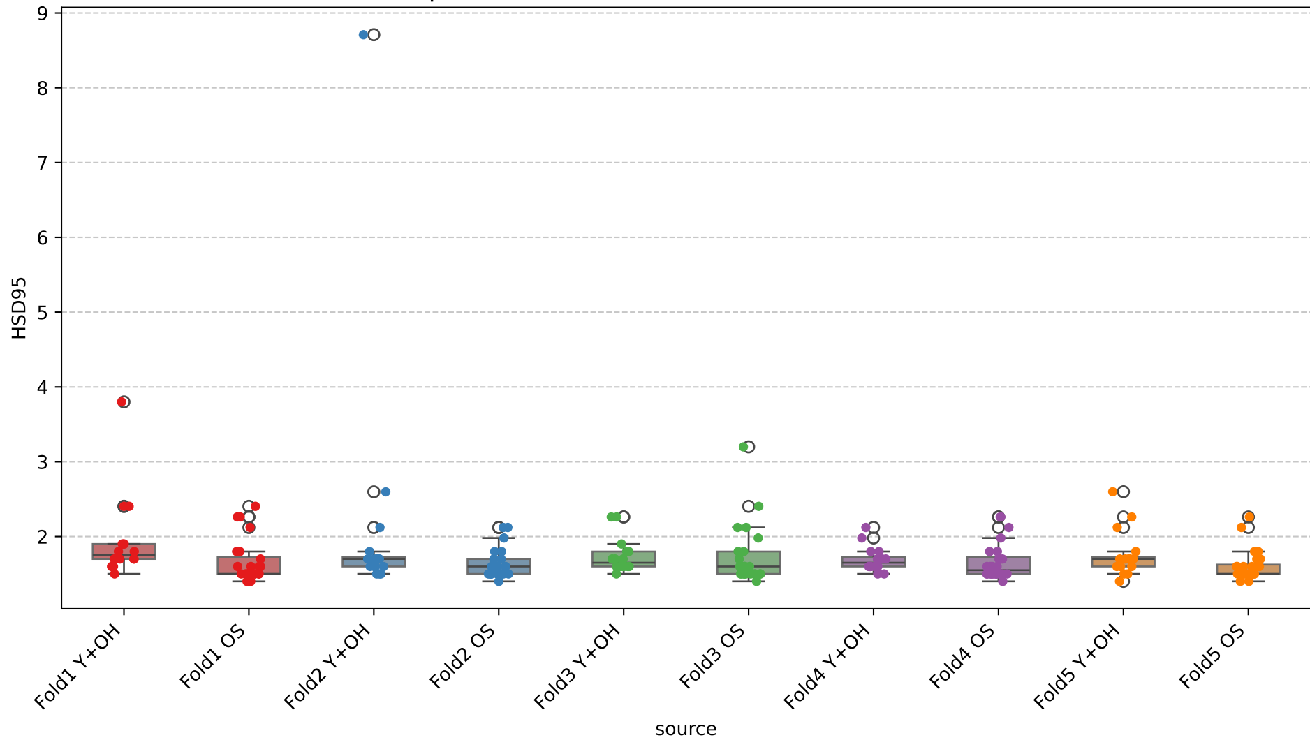
Boxplot of HSD95 across folds for two test sets
