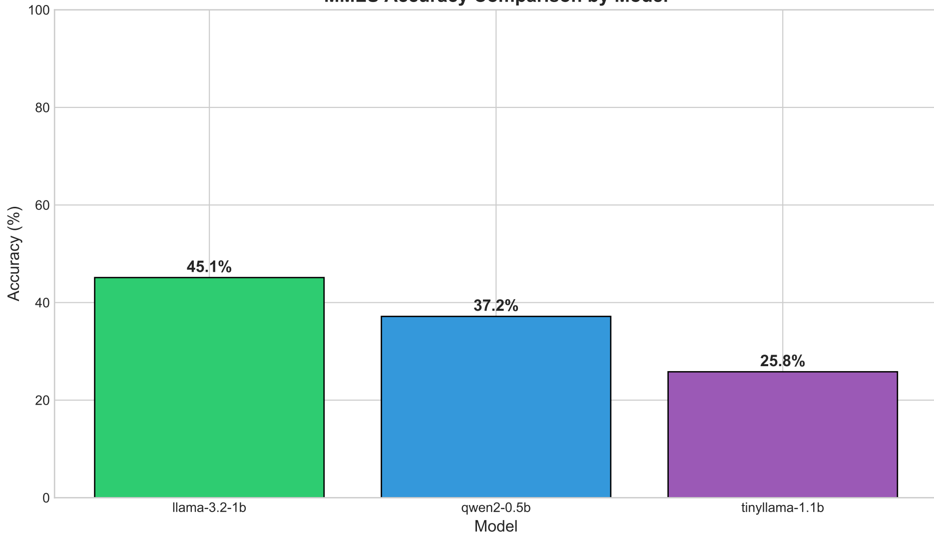
MMLU Accuracy Comparison by Model
