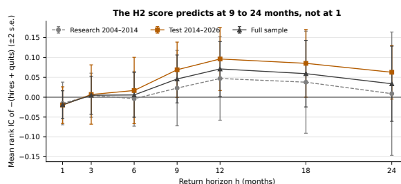
FIGURE 5. Post-hoc horizon profile of the H2 score: no one-month IC and a positive IC from 9 to 24 months, peaking at 12 (test +0.096, t = 2.43 ).
