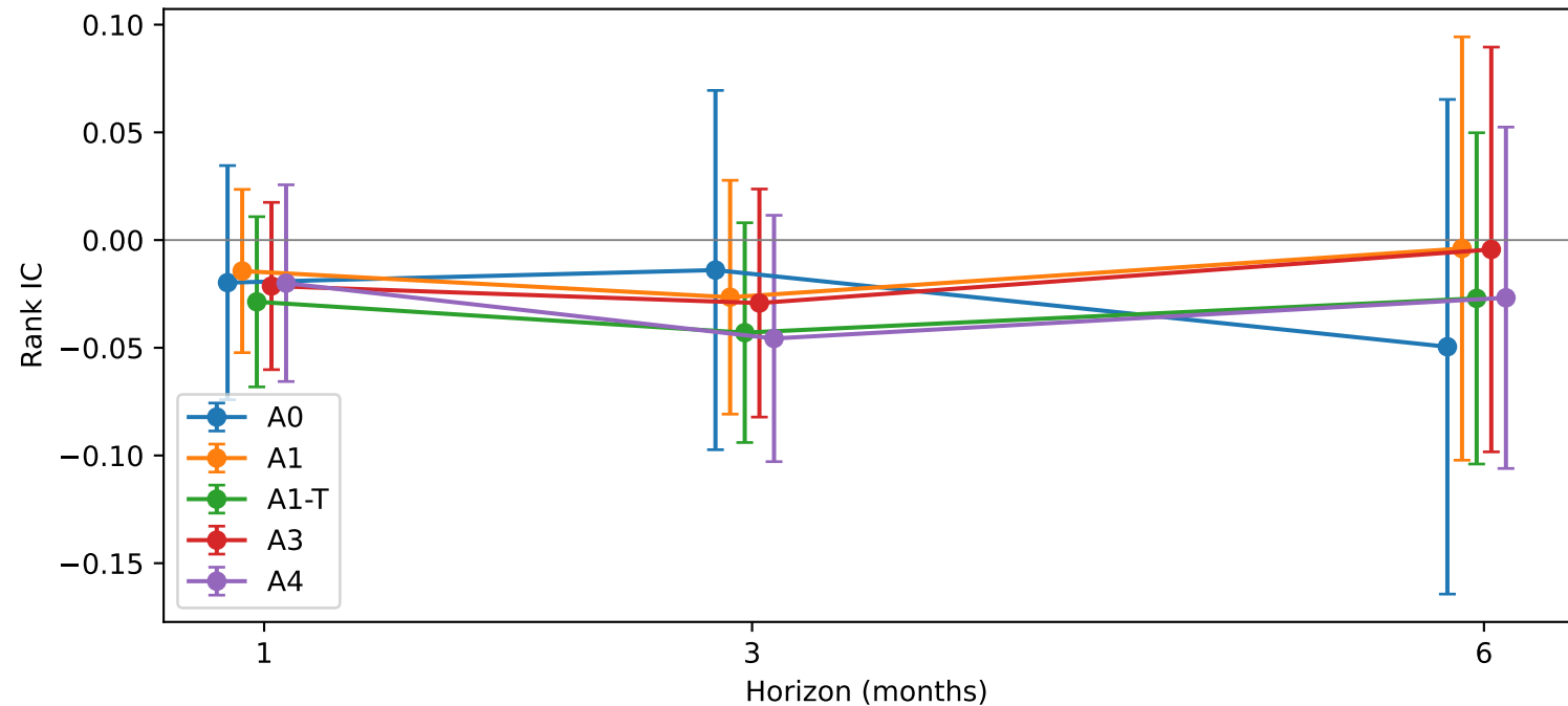
IC with 95% HAC intervals
