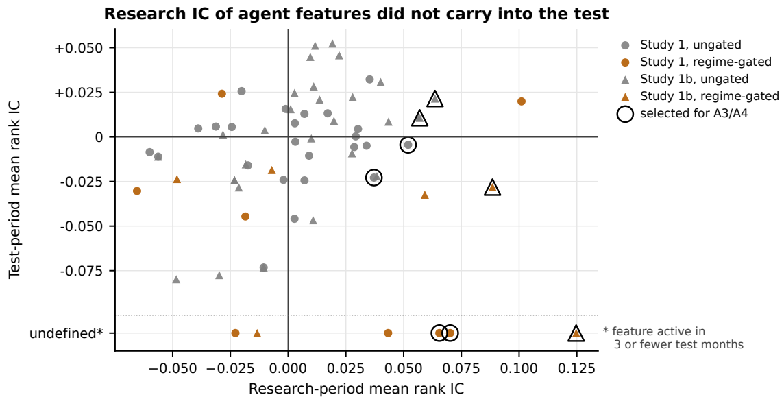
FIGURE 10. Research IC of agent features barely predicts their test IC; the selected regime-gated features were active in 3 test months.
