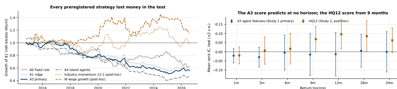
FIGURE 4. Left: every Study 1 strategy lost money in the test; the post-hoc wage-growth book gained until 2024 and gave much of it back. Right: horizon analysis in the test window; the A3 score has no IC at any horizon, the HQ12 score has none at one month and a positive IC from 9 to 24 months. CONFIRMATORY
