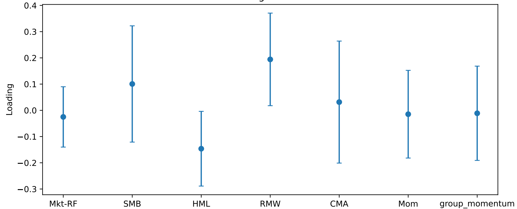
A3: factor loadings with HAC intervals
