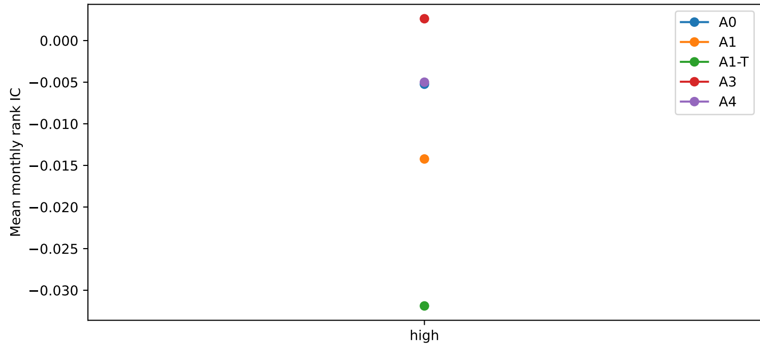
IC by expanding tightness tercile
